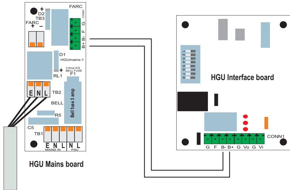
Cable to mains bell
